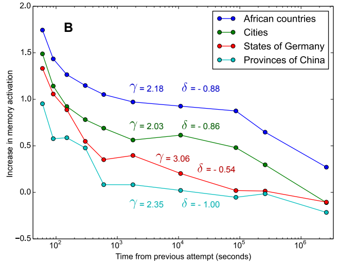
Figure 3: Time effect function and \gamma, \delta parameters fitted to filtered data: A) by estimated prior knowledge, B) by the type of a place.
