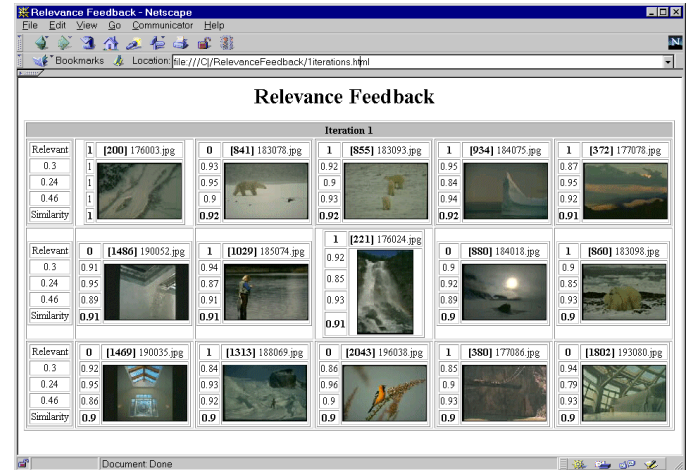
Fig. 7. The retrieval results after the relevance feedback
