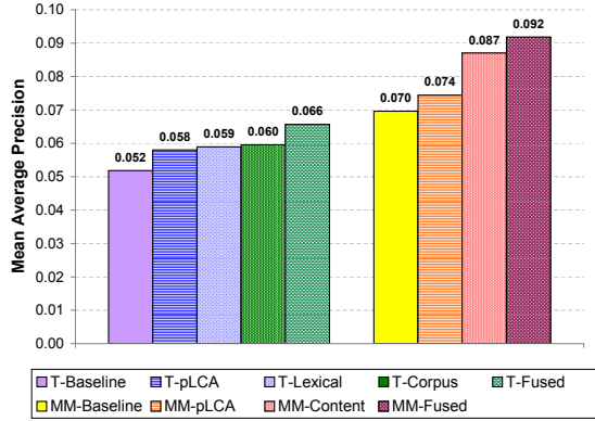
Figure 5: Performance evaluation of multimodal fusion on text-based retrieval systems and multi-modal retrieval systems. (left) MAP on TRECVID06 dataset and query topics, see Section 5.4 for definitions of the runs. (right) Relative improvements over text retrieval baseline for each of the 24 TRECVID06 queries.
