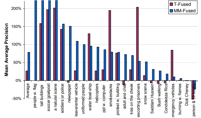
Figure 5: Performance evaluation of multimodal fusion on text-based retrieval systems and multi-modal retrieval systems. (left) MAP on TRECVID06 dataset and query topics, see Section 5.4 for definitions of the runs. (right) Relative improvements over text retrieval baseline for each of the 24 TRECVID06 queries.
