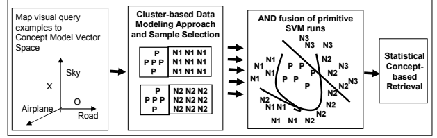
Figure 3: Statistical concept-based modeling.
