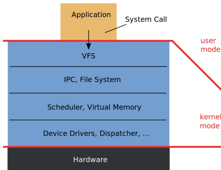
Monolithic Kernel based Operating System
