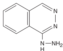
Hydralazine
