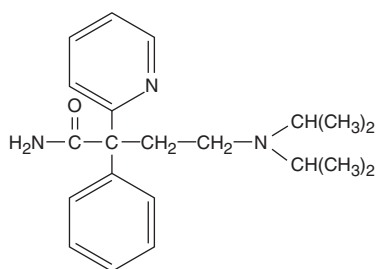
Disopyramide
