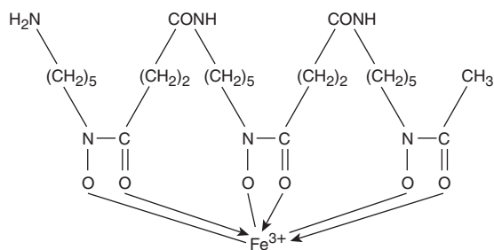
Ferroxamine
