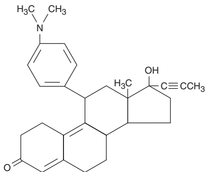
Mifepristone
