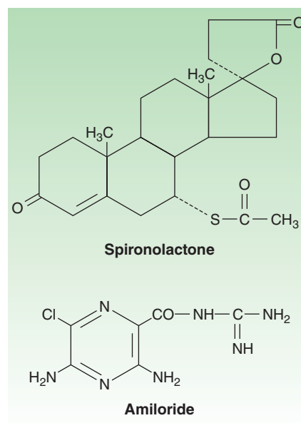
FIGURE 15–9 Potassium-sparing diuretics.
