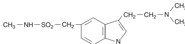
Sumatriptan
