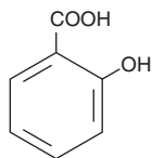
Salicylic acid
