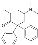
Methadone
