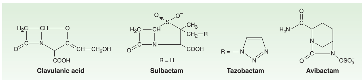
FIGURE 43–7 Beta-lactamase inhibitors.
