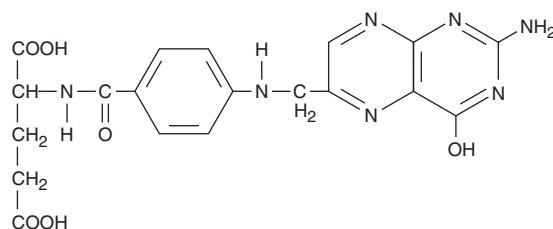
Folic acid
