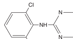
Clonidine
