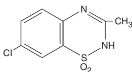
Diazoxide
