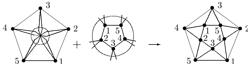
Figure 1: A double planar cover of K_5 , constructed by lifting its projective embedding into the sphere. The projection is determined by labels of vertices.
