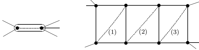
Figure 7: An illustration of a vertex splitting, and of a 3-step addition extension.
