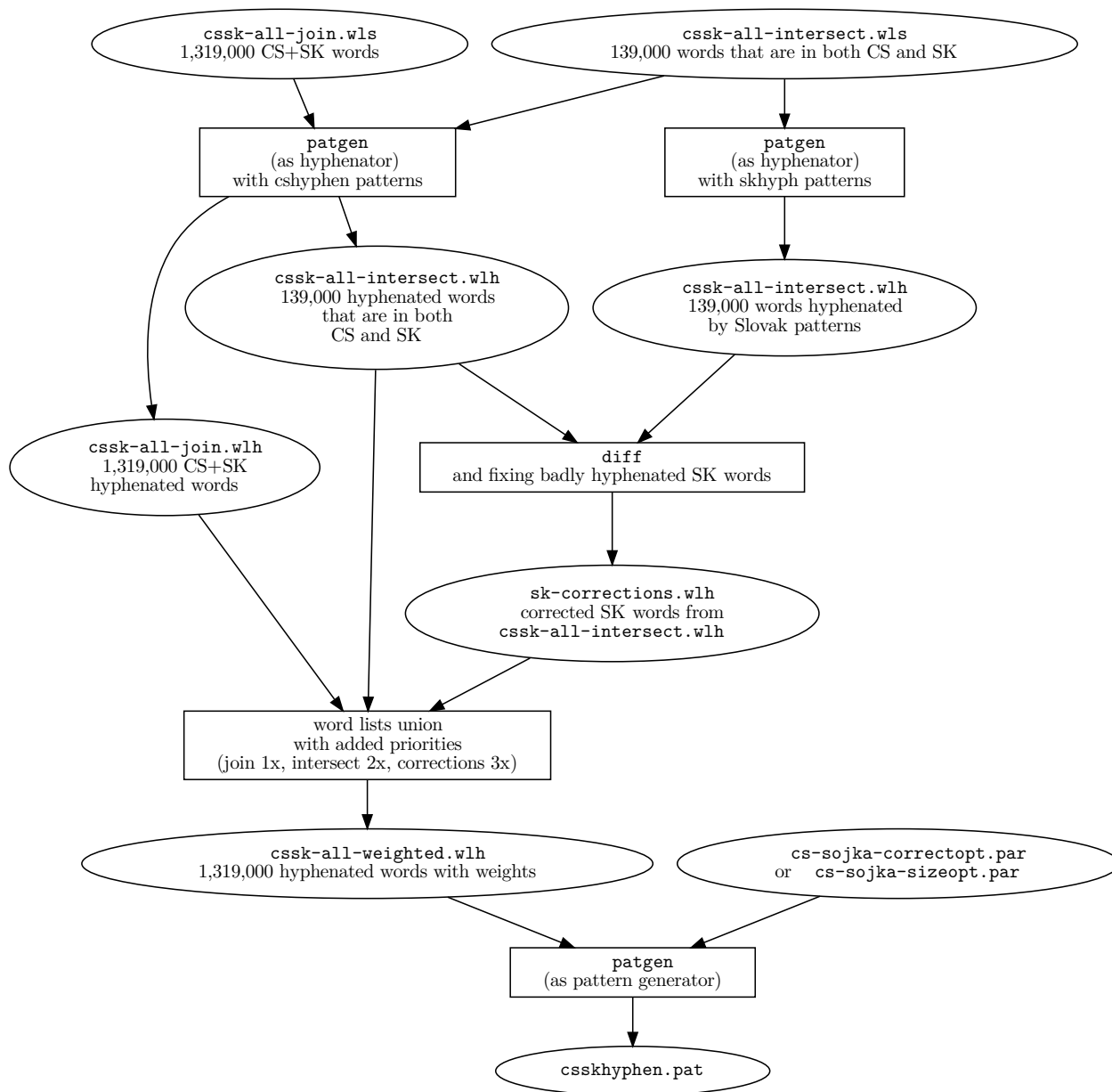
Figure 1: The whole pattern development workflow is showed above from top: a) Czech and Slovak word lists collection, [27] and intersection; b) bootstrapping hyphenated word lists with syllabic Czech patterns; c) checking and fixing by deploying rarely used patgen weighting for Slovak words common with Czech ones; d) generation of final patterns.
