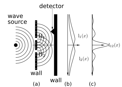
Figure 2: Experiments with waves
