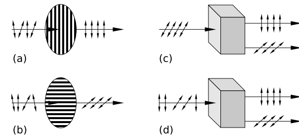
Figure: Photon polarizers and measuring devices
