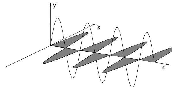
Figure: Linearly polarized photons - visualization
