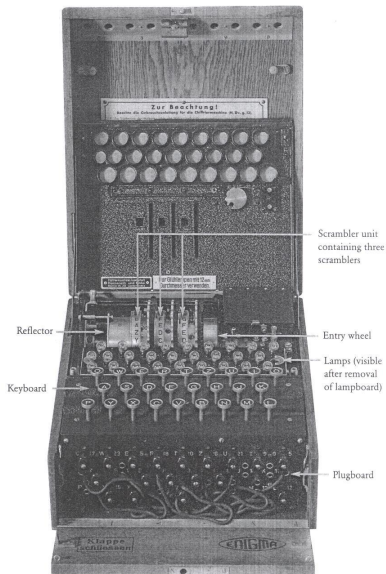
Figure 40 An Enigma machine with its top cover removed, showing the internal wiring.
