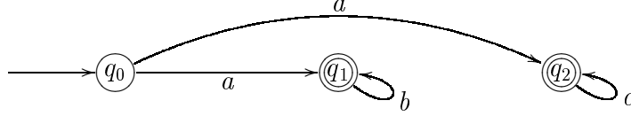
Fig. 1. Finite state automaton \mathcal{A} for the regular expression R ; edges are labelled with atomic propositions (i.e. formulas over AP ); q_1 and q_2 are accepting, q_0 is initial
