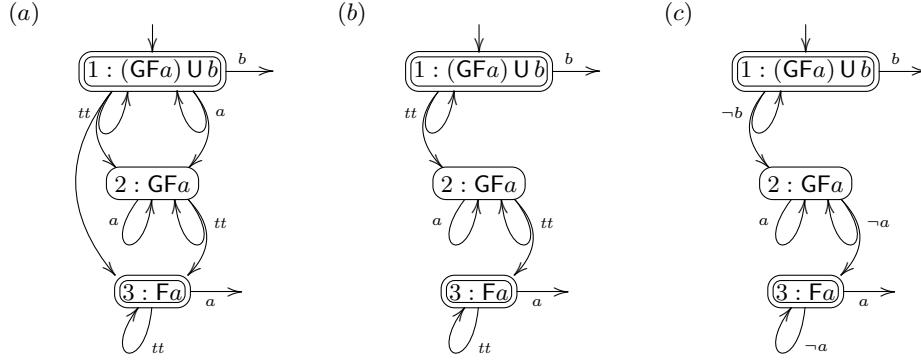
Fig. 1. VVAA for (GFa) U b generated by (a) the translation of [11], (b) our translation with suspension, and (c) our translation with suspension and further determinization.
