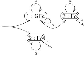
Fig. 3. A VVAA \mathcal{A}_\psi corresponding to \text{GF}a \wedge \text{F}b .
