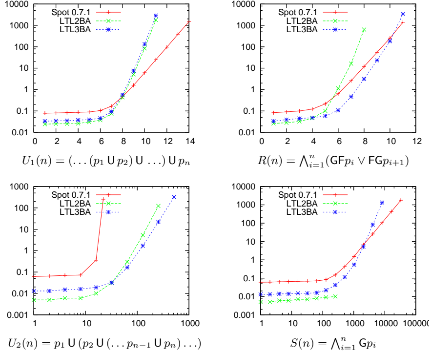
Fig. 10. Running times of LTL to BA translators on parametric formulae of [16] (the vertical axes are logarithmic and represent time in seconds, while the horizontal axes are linear or logarithmic and represent the parameter n ).
