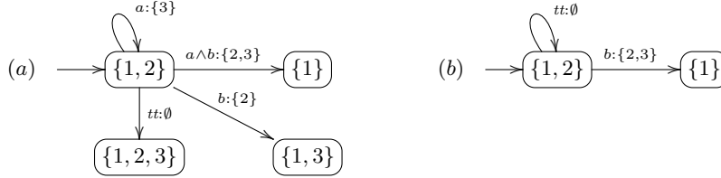
Fig. 8. Transitions leading from state \{1, 2\} in the TGBA constructed from the VWAA of Figure 3 by (a) the translation of [11] and by (b) our translation with suspension.
