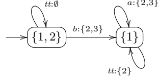
Fig. 4. A TGBA \mathcal{G}_\psi corresponding to the VVAA of Figure 3.
