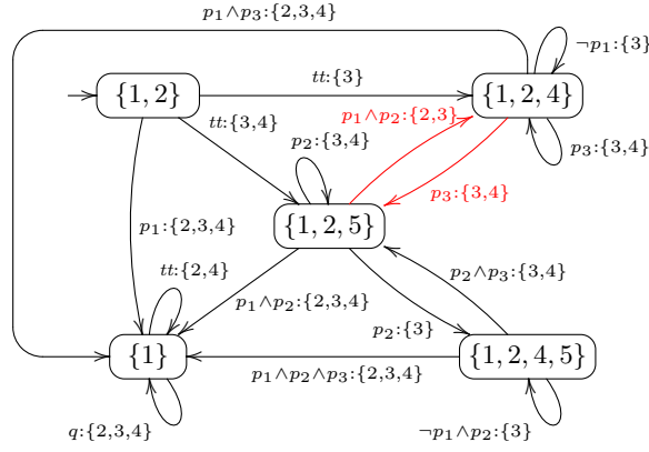
Fig. 6. A TGBA \mathcal{G}_\varphi corresponding to the VVAA of Figure 5 constructed using original definition of accepting sets.
