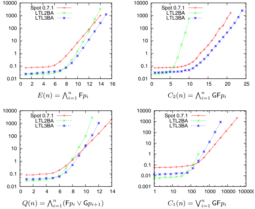
Fig. 11. Running times of LTL to BA translators on another parametric formulae of [16] (the vertical axes are logarithmic and represent time in seconds, while the horizontal axes are linear or logarithmic and represent the parameter n ).
