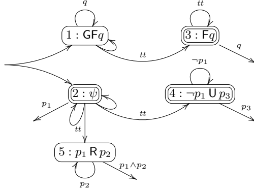
Fig. 5. A VVAA \mathcal{A}_\varphi corresponding to formula \varphi = \psi \wedge \text{GF}q , where \psi = (\text{X}((p_1 \text{R} p_2) \vee (\neg p_1 \text{U} p_3))) \text{U} p_1 .
