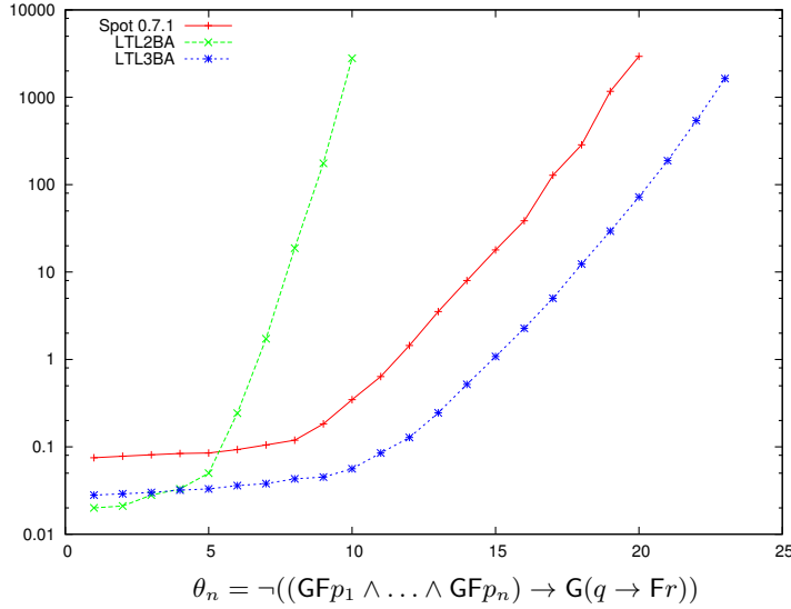
Fig. 9. Running times of LTL to BA translators on parametric formula \theta_n of [11] (the vertical axis is logarithmic and represent time in seconds, while the horizontal axis is linear and represent the parameter n ).
