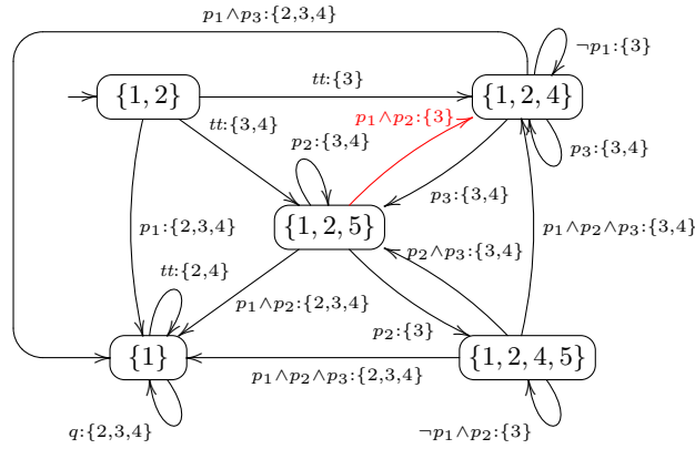
Fig. 7. A correct TGBA \mathcal{G}'_\varphi corresponding to the VVAA of Figure 5 constructed using modified definition of accepting sets.
