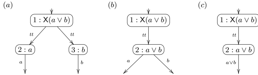
Fig. 2. VVAA for X(a \vee b) generated by (a) the translation of [11], (b) our translation with suspension, and (c) the translation with suspension and further determinization.
