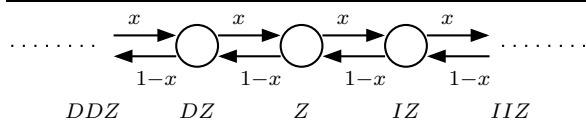
Figure 1. Bernoulli random walk as a pBPA
