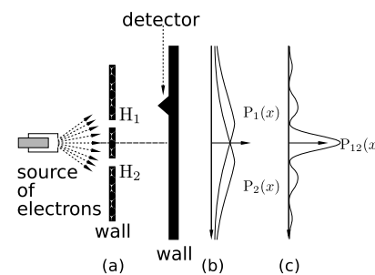
Figure 3: Two-slit experiment
