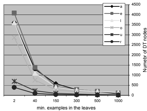
Fig. 4. Sizes of DT from Table 3
