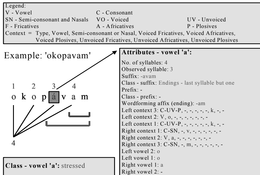
Fig. 1. Attributes for the third vowel ('o') of Slovenian word "okopavam" (engl. "I earth up")
