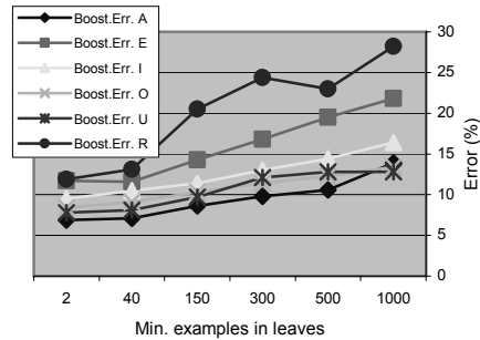
Fig. 3. Boosted DT error on different pruning parameters
