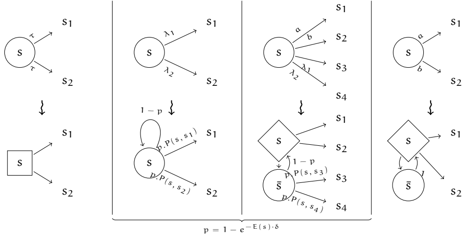
Figure 1: Four gadgets for transforming a CE game into a discrete game. The upper part shows types of states in the original CE game, the lower part shows corresponding gadgets in the transformed discrete game. In the lower part, the square-shaped, diamond-shaped and circle-shaped vertices belong to V_{\square} , V_{\diamond} and V_{\circ} , respectively. Binary branching is displayed only in order to simplify the figure.
