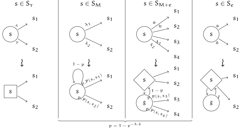
Figure 2: Four gadgets for transforming a CE game into a discrete game. The upper part shows types of states in the CE game, the lower part shows corresponding gadgets in the discrete game. In the lower part, the square-shaped vertices belong to player \square , the diamond-shaped vertices to player \diamond and the circle-shaped vertices to player \circ .
