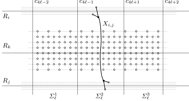
Fig. 5. An illustration to Lemma 4.8
